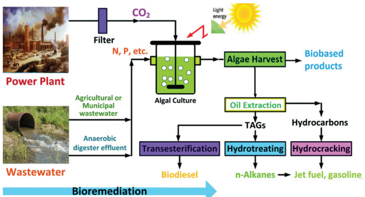
Figure 9. Using of \text{CO}_2 (industrial produced) in enrichment of algal biomass production.
