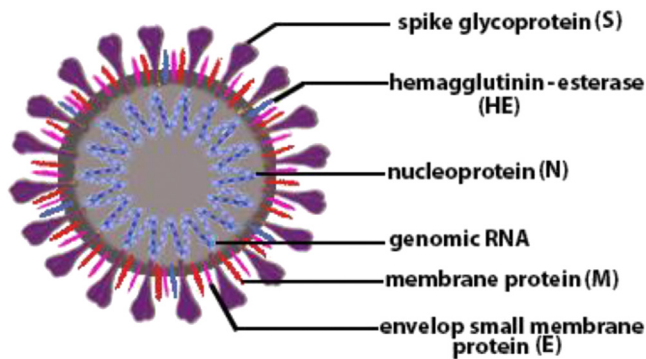
Figure 1. Structure of SARS-CoV-2.
