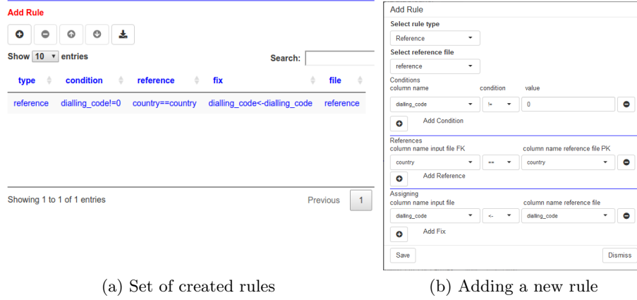
Fig. 5: Reference rule example.
