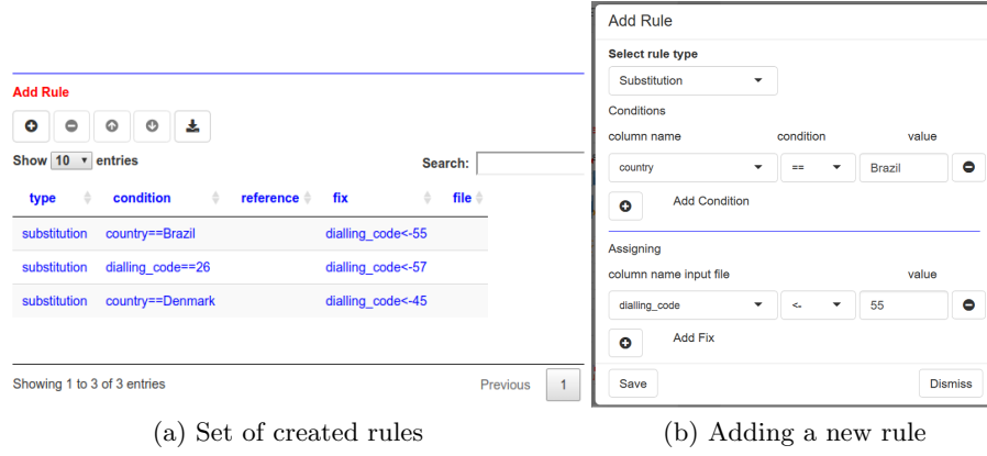
Fig. 4: Substitution rule example.
