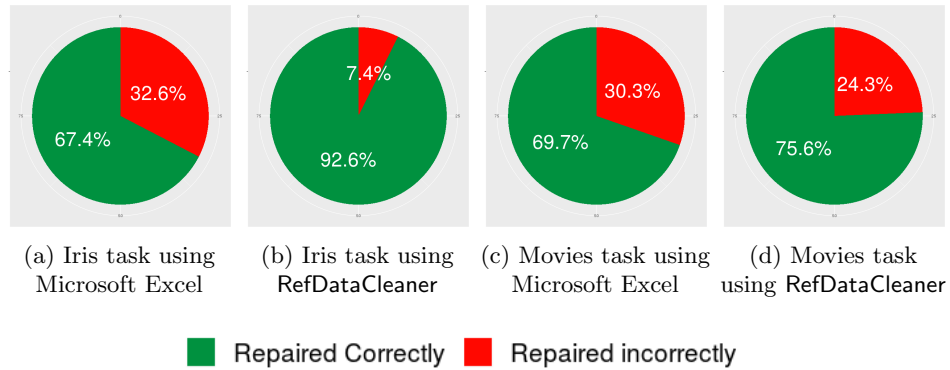
Fig. 9: Data repair accuracy.
