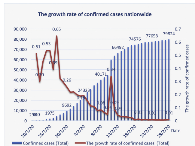
Fig. 2. Total number of confirmed cases nationwide. Up to 29 Feb 2020, the confirmed cases reached 79,824 in China, and the growth rate of confirmed cases is 0.01% nationwide.
