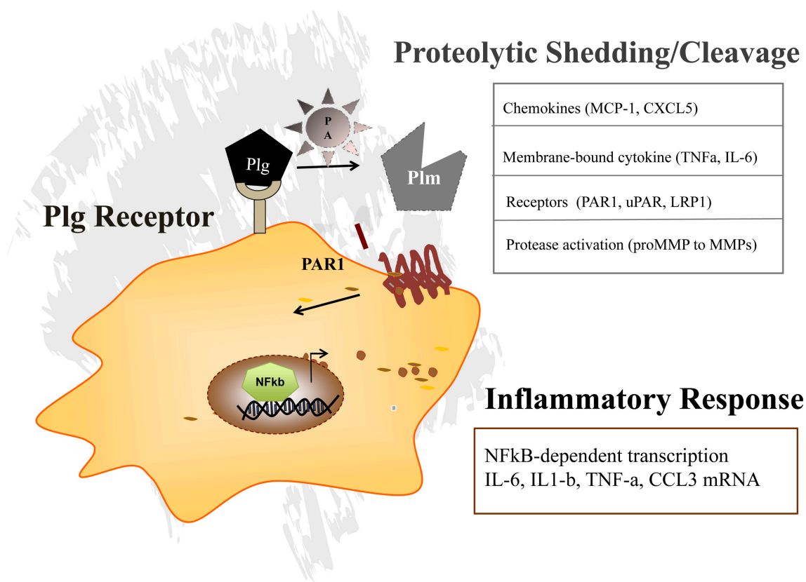
Fig. 3. Plasminogen receptors localize plasmin generation to the pericellular space, thereby promoting signaling receptor shedding (e.g. PAR1). Plg receptors present Plg and enhance plasminogen activator (PA) mediated pericellular plasmin (Plm) generation. The proteolytic activity of Plm is required to activate PAR1 signaling or for shedding or cleavage of other proteases (MMPs) as well as in signaling by other molecules like cytokines or cellular receptors.
