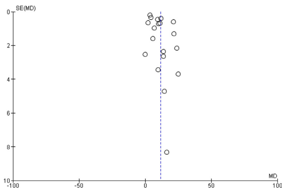
Fig. 5. Funnel plot.
