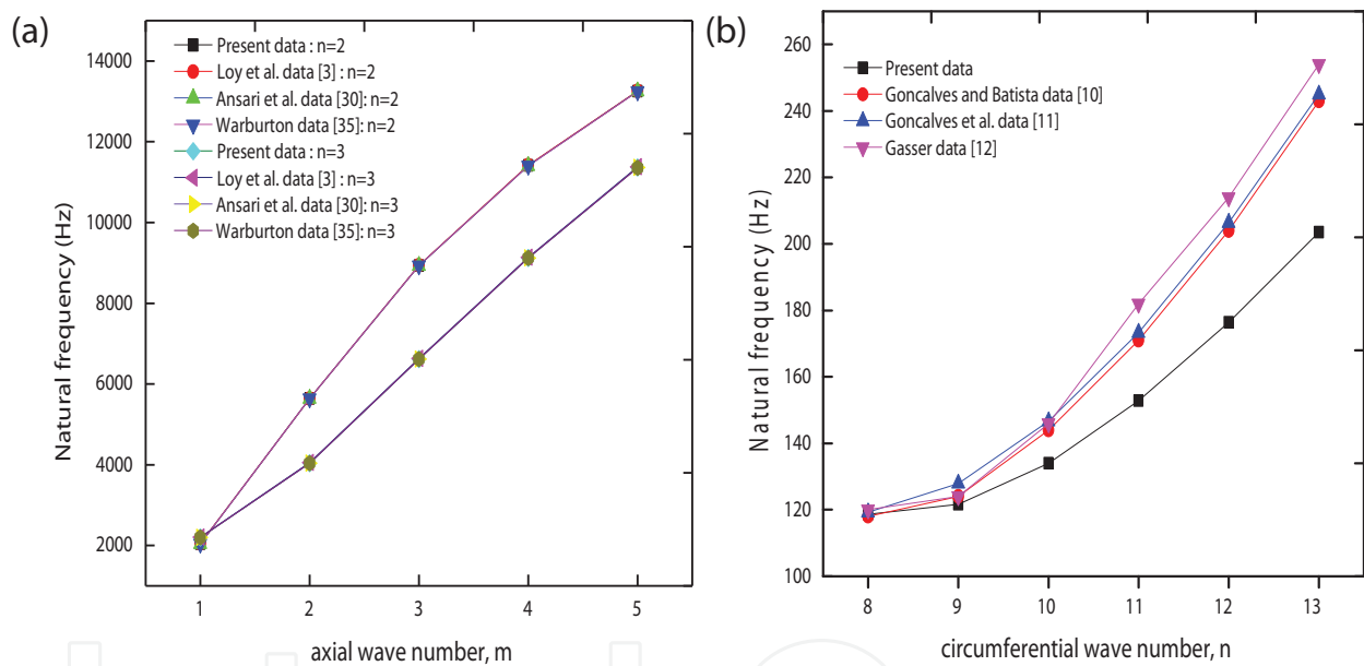
Figure 2. (a) Comparison of natural frequencies (Hz) for a simply supported CS ( L = 8 in, h = 0.1 in, R = 2 in, E = 30 \times 10^6 lbf in ^{-2} , \nu = 0.3 , \rho = 7.35 \times 10^{-4} lbf s ^2 in ^{-4} ). (b) Comparison of natural frequencies (Hz) for a fluid-filled CS ( m = 1, L = 0.41 m, h = 0.001 m, R = 0.3015 m, E = 2.1 \times 10^{11} N/m ^2 , \nu = 0.3 , \rho = 7850 kg/m ^3 ).
